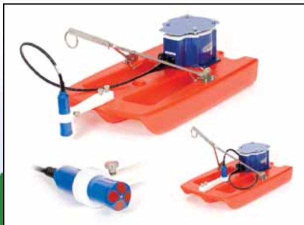
The StreamPro's transducer can be towed from the front or middle of the float, or can be removed and hand-held in the water for applications such as under-ice flow measurements.
